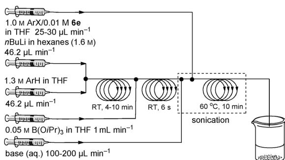
Figure 4. Continuous-flow setup for the lithiation/borylation/Suzuki–Miyaura cross-coupling sequence of heteroarenes with aryl halides.
