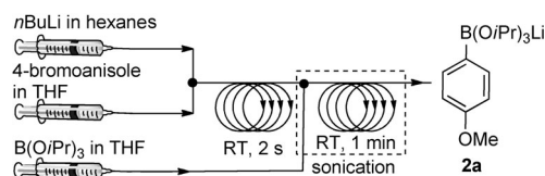
Figure 1. Continuous-flow setup for the room-temperature lithiation/borylation of 4-bromoanisole.
